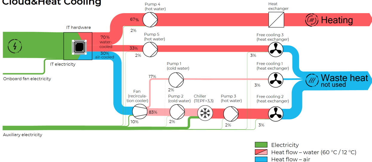
Illustration 3: Energy flow diagram - classic air cooling vs. Cloud&Heat Cooling
